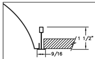
Lay-In Ceiling with 9/16 T grid fixture lies flush with ceiling tile.
