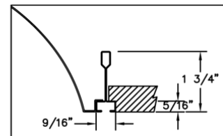
Lay-In Ceiling with Slot-Grid T fixture lies flush with ceiling tile.
