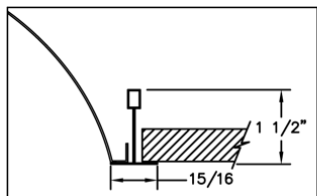
Lay-In Ceiling with 15/16 T grid fixture lies flush with ceiling tile.
