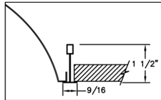
Lay-In Ceiling with 9/16 T grid fixture lies flush with ceiling tile.
