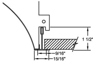
'T'- Flat Grid Tee 9/16" & 15/16"
