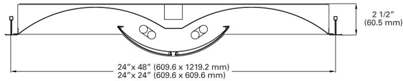
Size: 2x2 & 2X4
