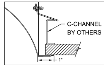
'F'- Sheet Rock Ceiling
