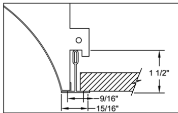
'T'- Flat Grid Tee 9/16" & 15/16"
