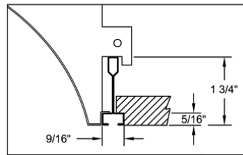
'S'-Slot Grid Tee
